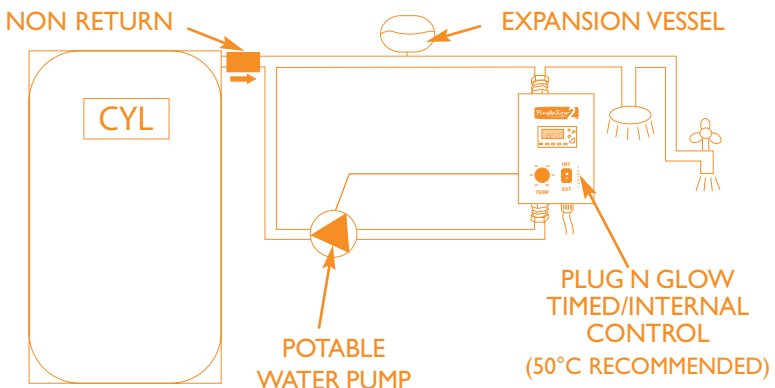
Figure 3 - SECONDARY RETURNS WITH HEAT PUMP AND THERMAL STORE CYLINDERS
